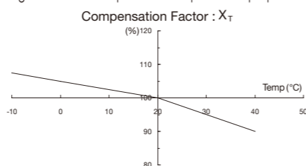
<Fig. 2. Mounting condition compensation>
